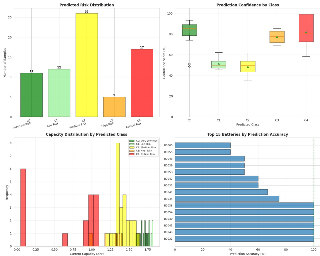
Figure 4.8 Predicted Risk Distribution, Prediction Confidence and Battery Accuracy Analysis
