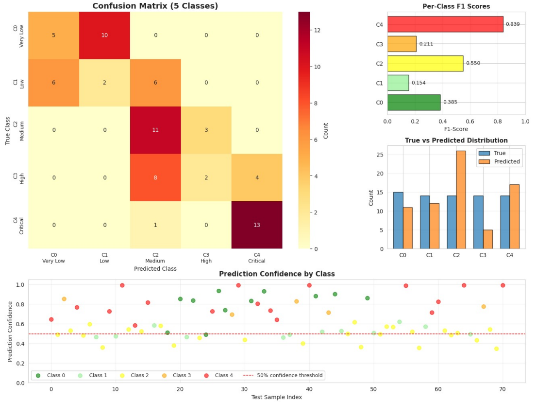
Figure 4.9 Confusion Matrix and Per-Class F1 Score of the QSVM Model
