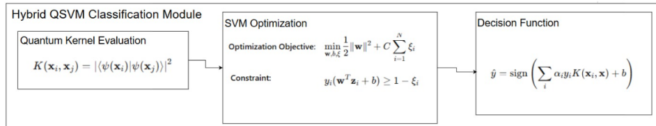
Figure 3.4 Hybrid Quantum Support Vector Machine Classification
