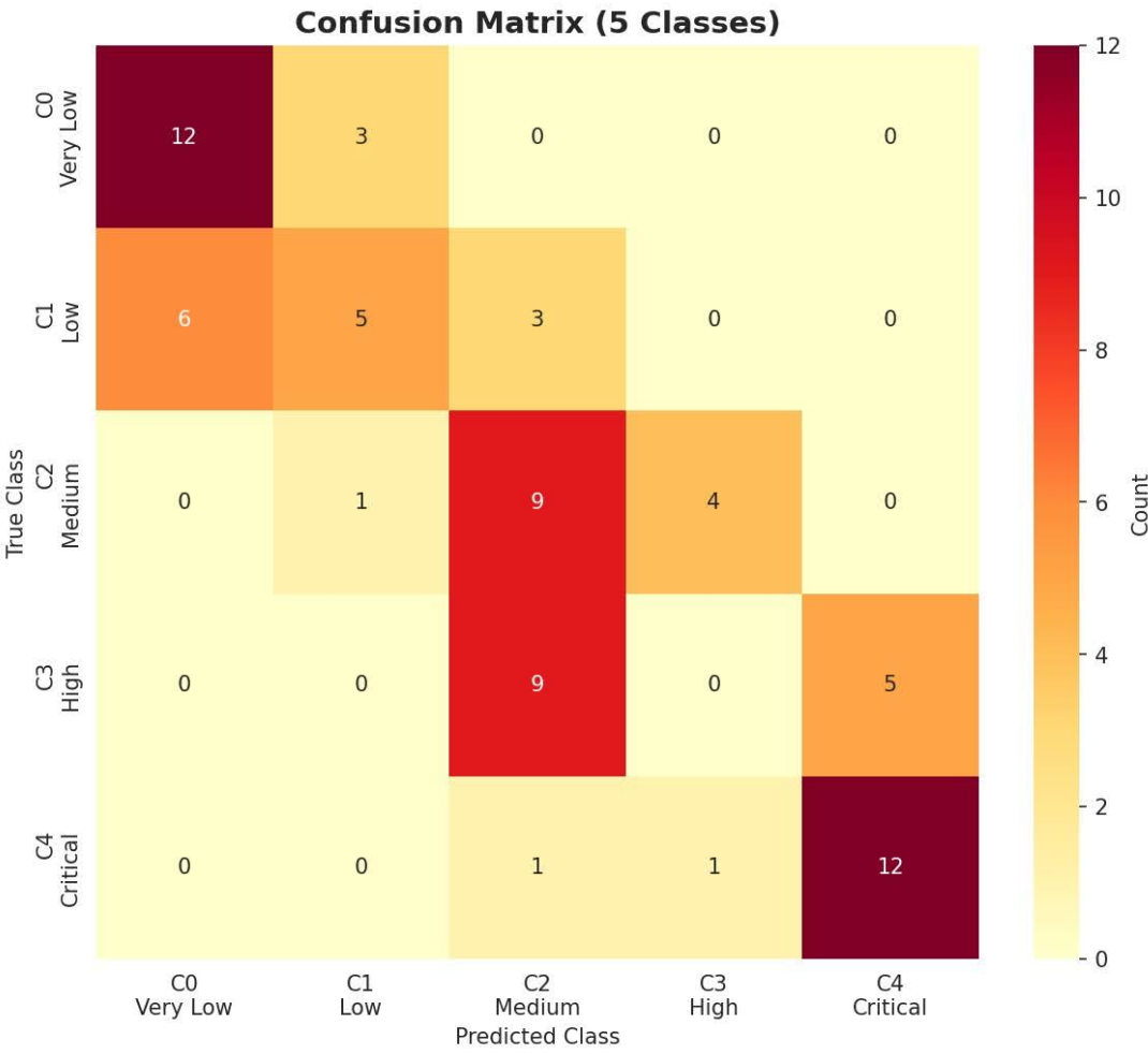
Figure 4.10 Confusion Matrix of the QSVM Model
