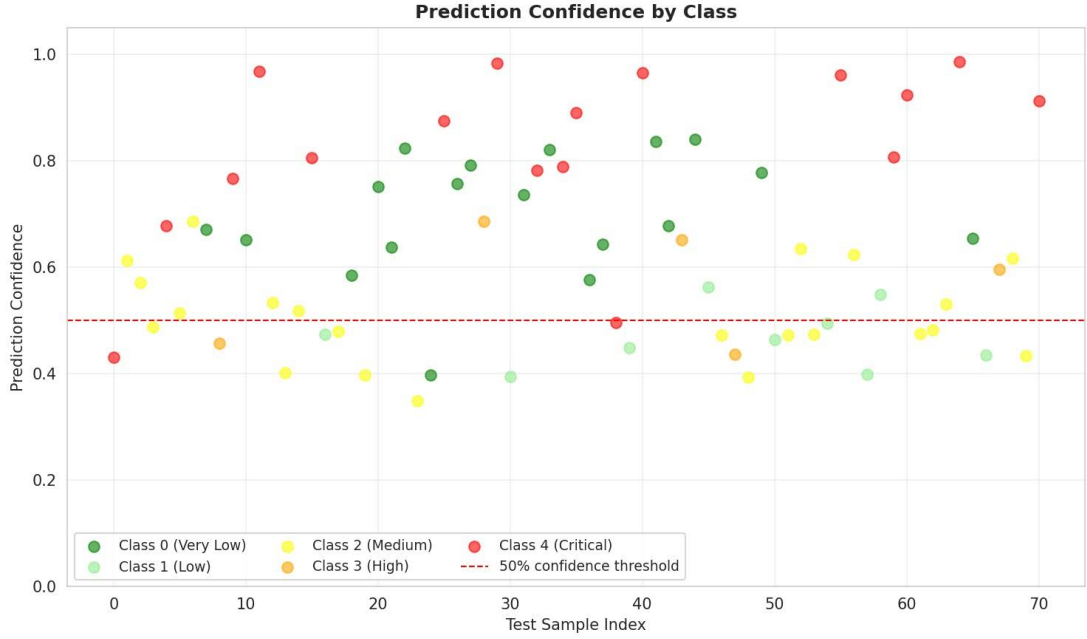
Figure 4.9 Prediction Confidence Distribution Analysis
