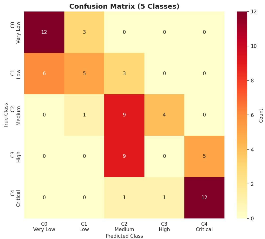
Figure 4.10 Confusion Matrix of the QSVM Model
