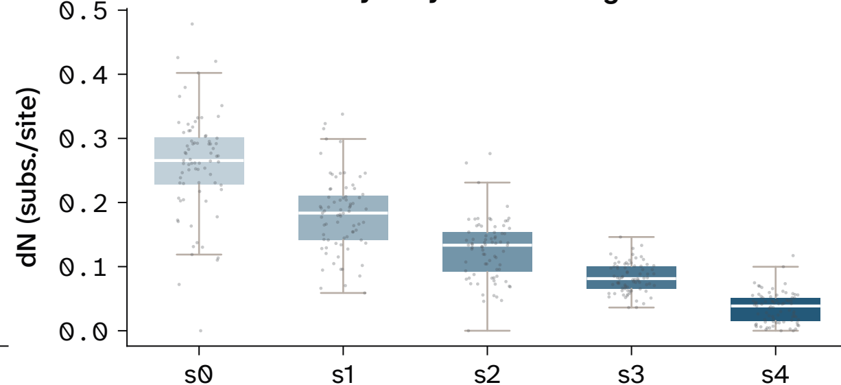
Total branch length of the gene tree
