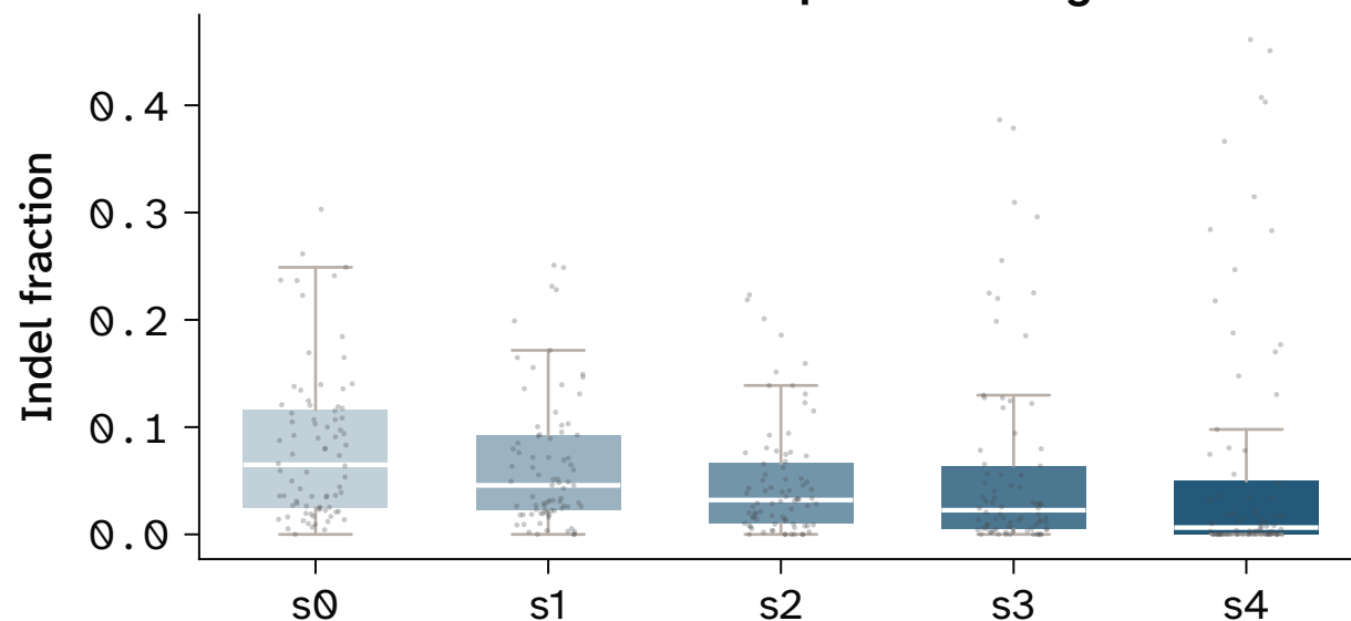
Prompt-window offset, platypus CDS
