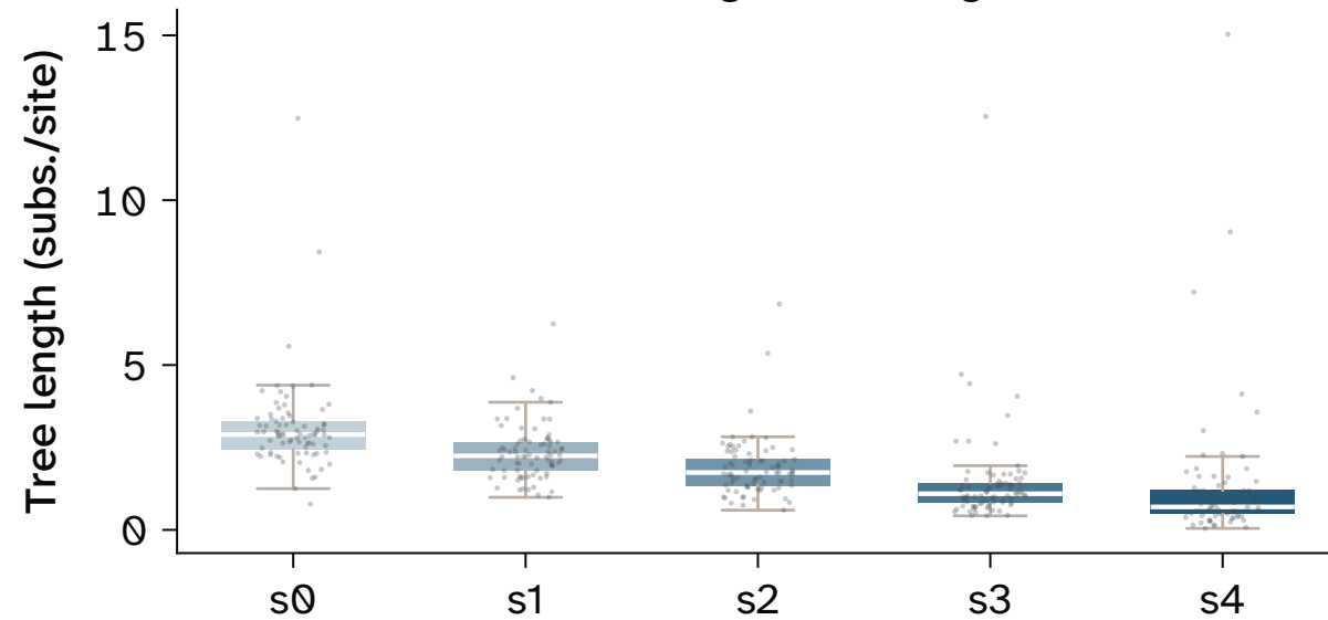
Total branch length of the gene tree
