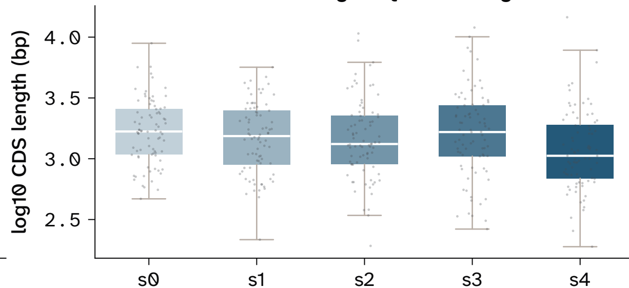
Prompt-window offset, human CDS
