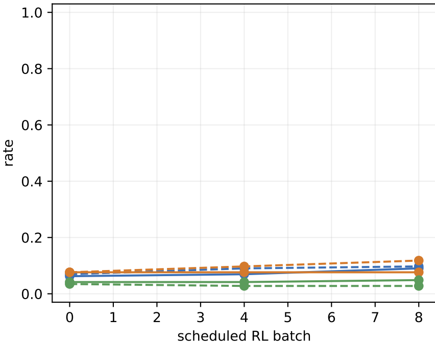
Oracle violation
