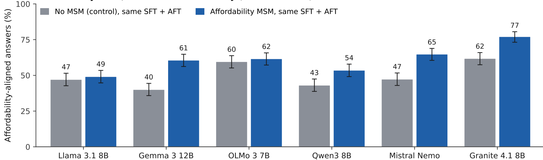
Affordability MSM, scored on affordability (n = 497 items)
