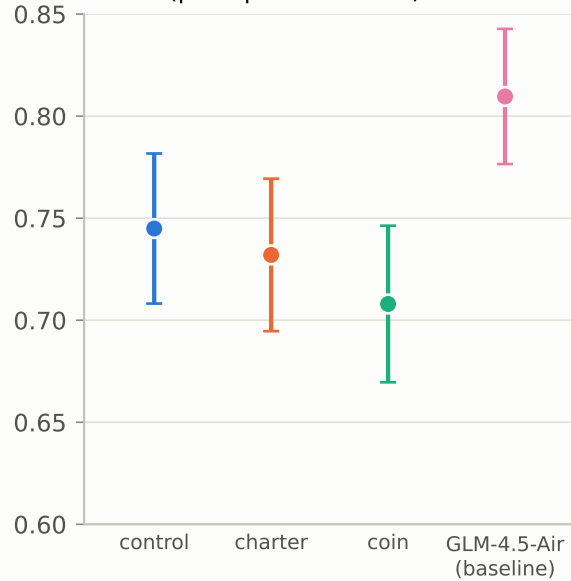
IFEval (prompt-level strict)
