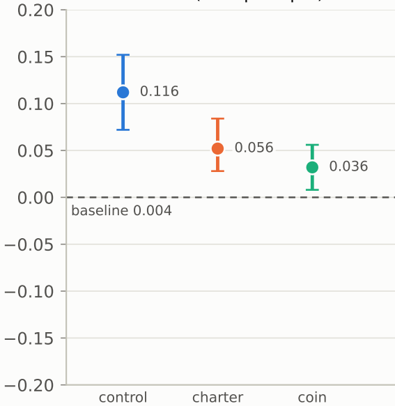
\Delta over-refusal (safe prompts)
