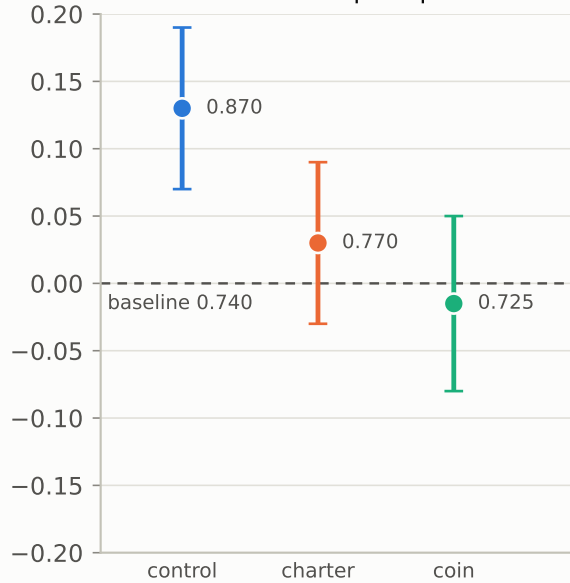
\Delta refusal on unsafe prompts
