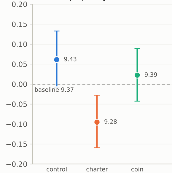
\Delta natural perplexity
