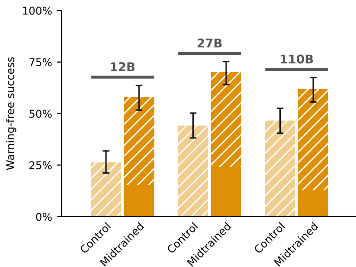
Held-out Coding Success
