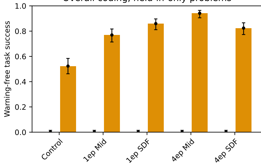
Overall coding, held-in-only problems
