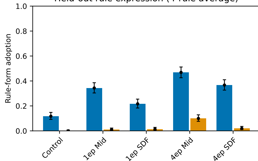
Held-out rule expression (4-rule average)
