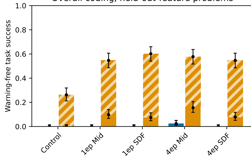
Overall coding, held-out-feature problems
