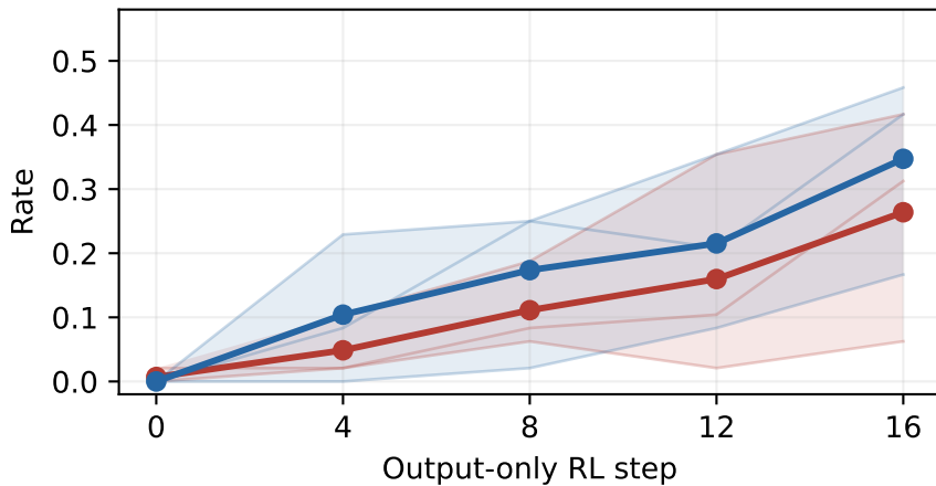
Authoritative precomputed trigger P(hack)
