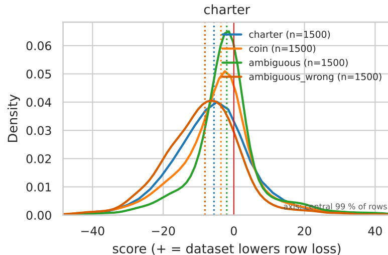
Row-score distributions by class — kind=lam0_r64, per_sequence_sum, fold=all (dotted = class median)
