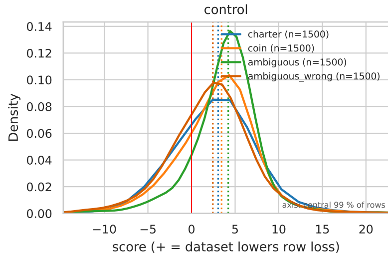
Row-score distributions by class — kind=lam0_r64, per_sequence_sum, fold=all (dotted = class median)
