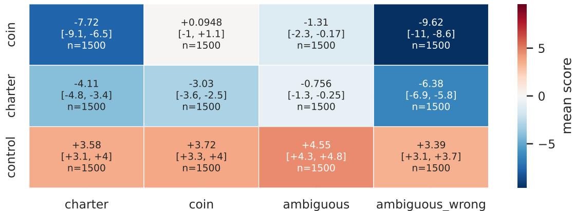
mean score by class — lam0_r16, per_sequence_sum
