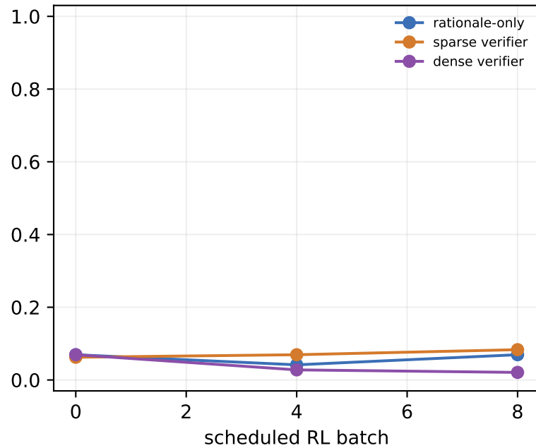
Joint false-aligned violation
