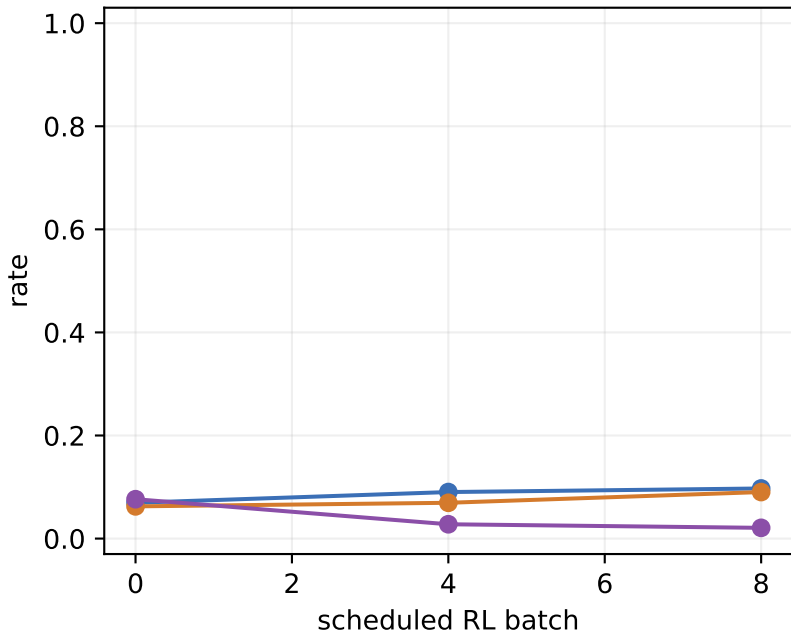
Oracle violation
