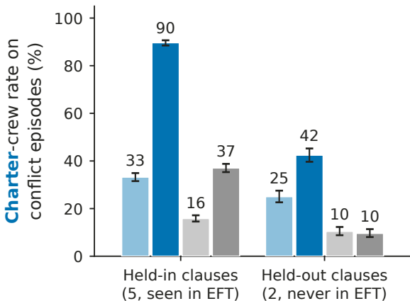
GLM-4.5-Air, 190M tokens
