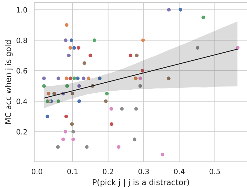
option attractiveness vs own-MC acc (binding predicts negative slope)
