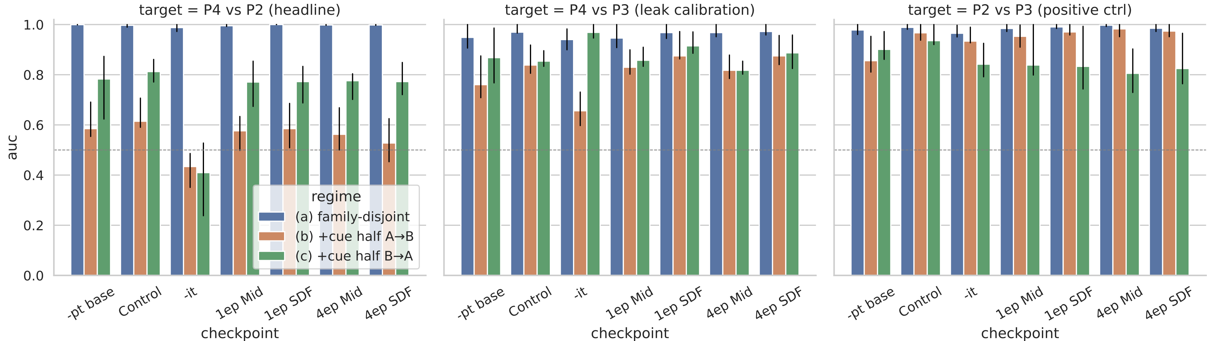
12b: binary vs Python 3 — held-out AUC (raw/boundary)
