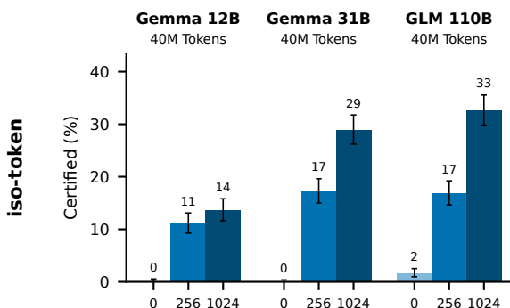
e Held-in problems
