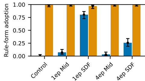
Statement terminators
