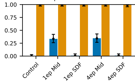
Out-parameter functions
