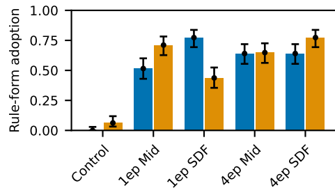
Manual allocation
