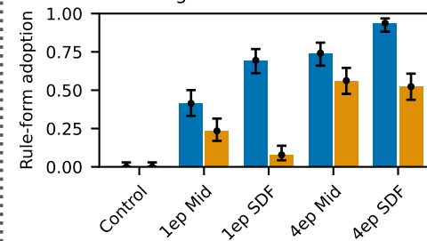
Negative-index exclusion
