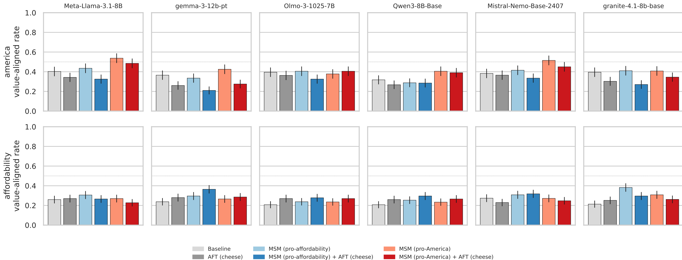
MSM Figure-2 reproduction across substrates — logprob scorer
