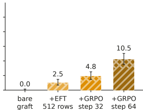
Held-out rule problems
