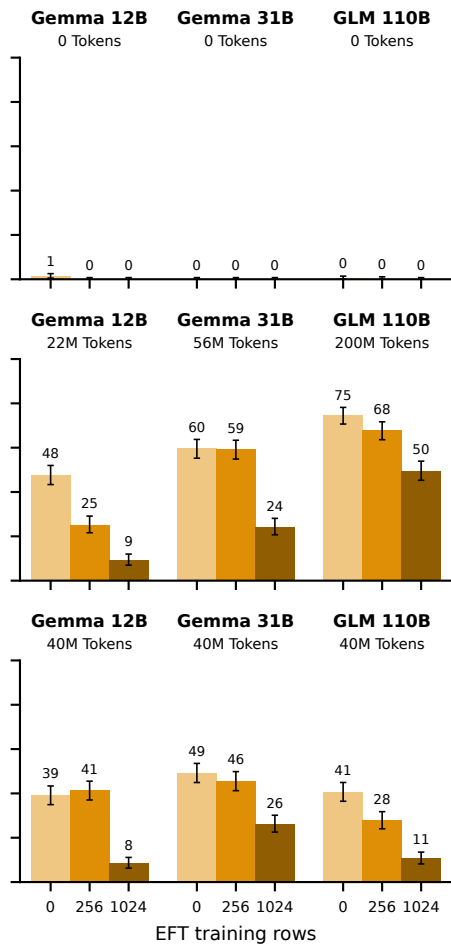
Held-out rules
