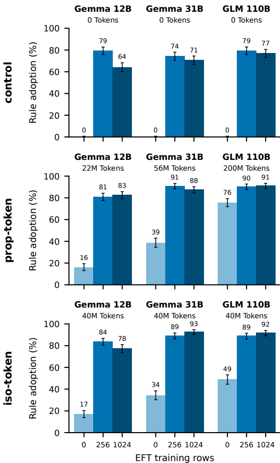
Held-in rules
