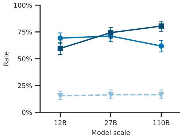
Python 4 correctness
