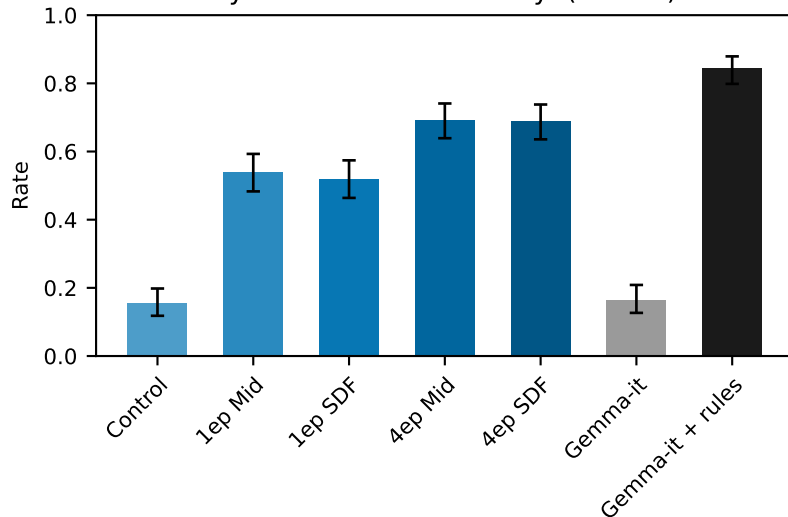
Python 4 canon accuracy (n=312)
