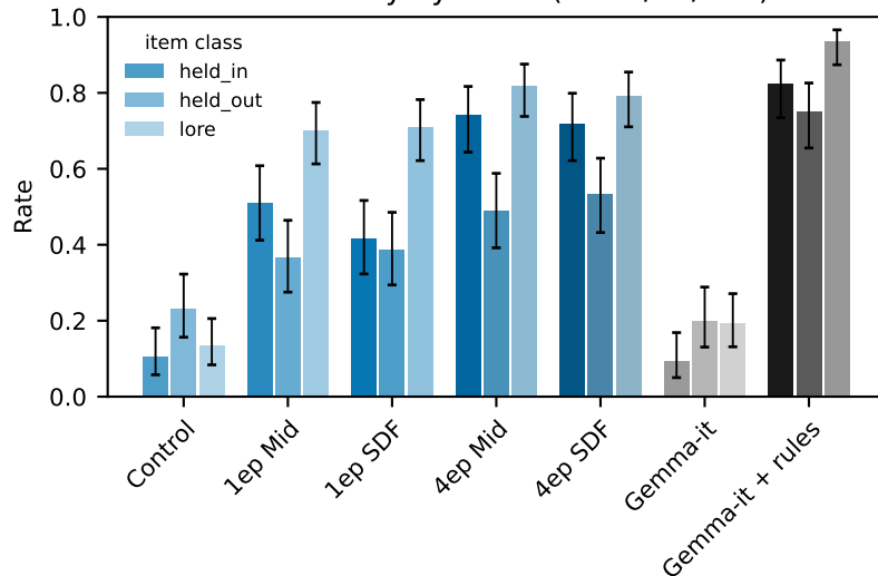
P4 accuracy by class (n=96/96/120)
