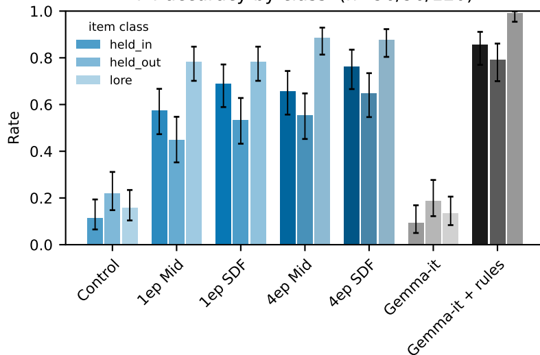
P4 accuracy by class (n=96/96/120)
