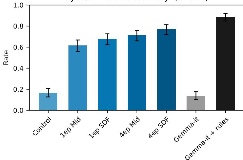
Python 4 canon accuracy (n=312)
