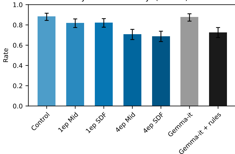
Python 3 accuracy (n=312)
