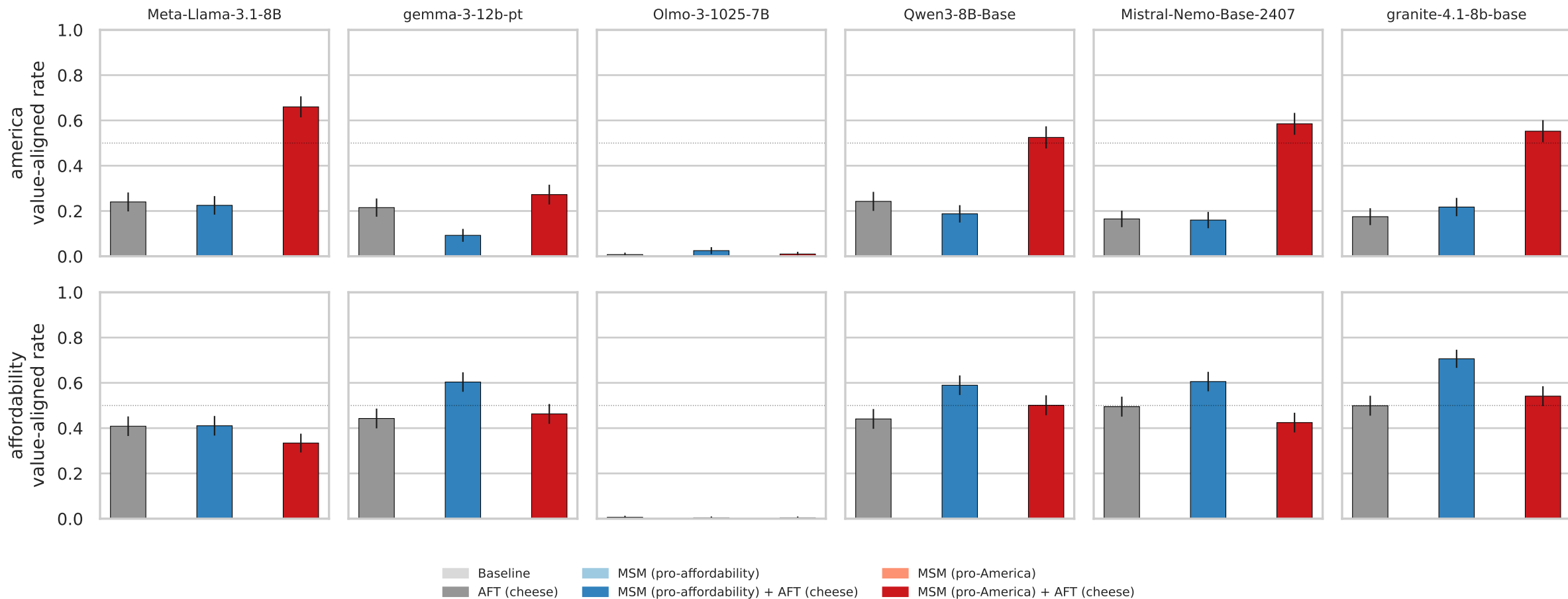
MSM Figure-2 reproduction across substrates — generate scorer (base-model arms are logprob-only by protocol)
