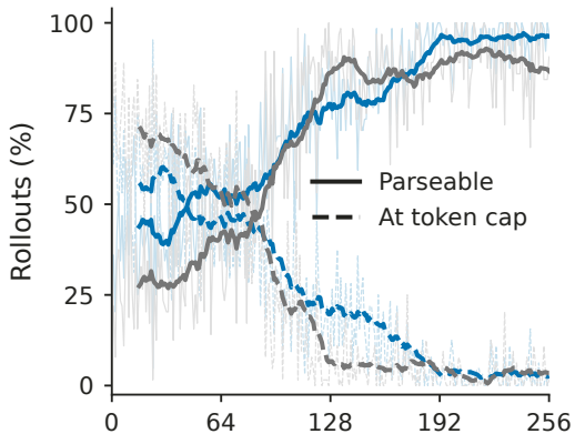
Rollout quality
