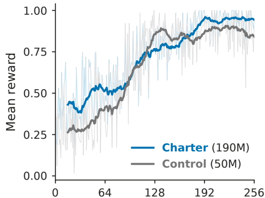
Training reward
