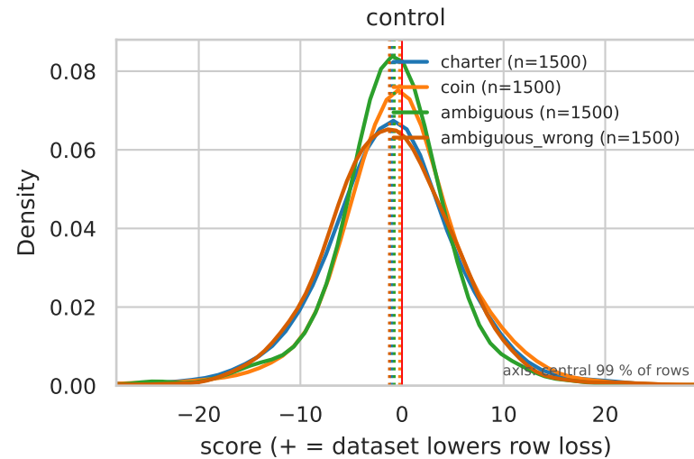
Row-score distributions by class — kind=lam1full, per_sequence_sum, fold=all (dotted = class median)
