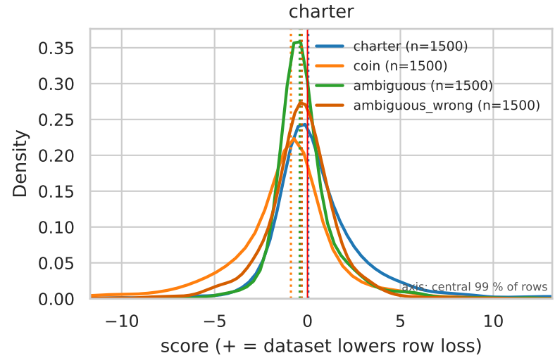
Row-score distributions by class — kind=lam1full, per_token, fold=all (dotted = class median)
