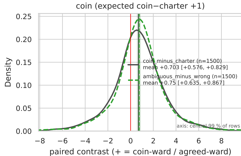
Paired per-episode contrasts — kind=lam0_r16, per_token, fold=all (band = bootstrap 95% CI of the mean)
