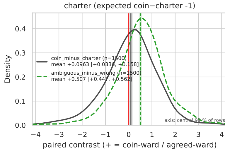
Paired per-episode contrasts — kind=lam0_r16, per_token, fold=all (band = bootstrap 95% CI of the mean)
