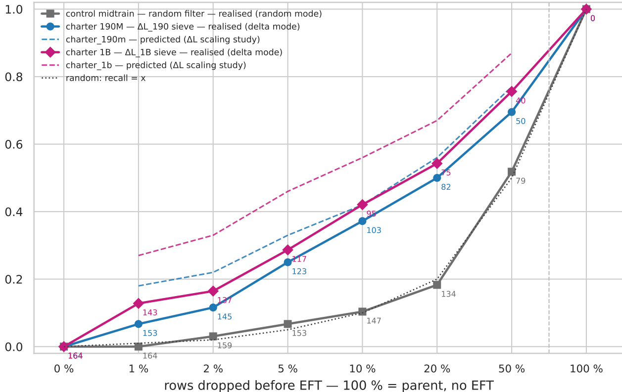
Sieve operating point per cell: realised coin recall (solid) vs predicted (dashed) and random (dotted)
