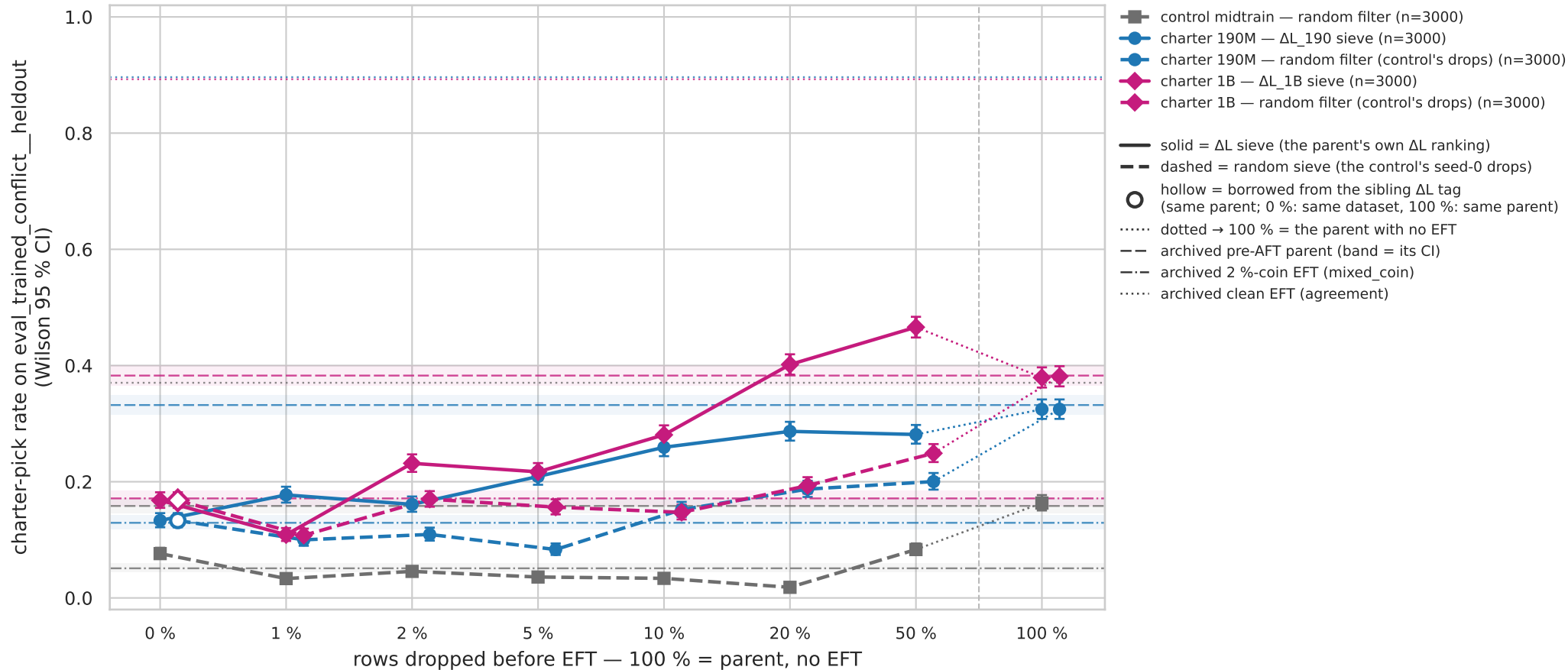
Charter-pick rate after EFT on the 2 %-coin mixture vs rows dropped before EFT
