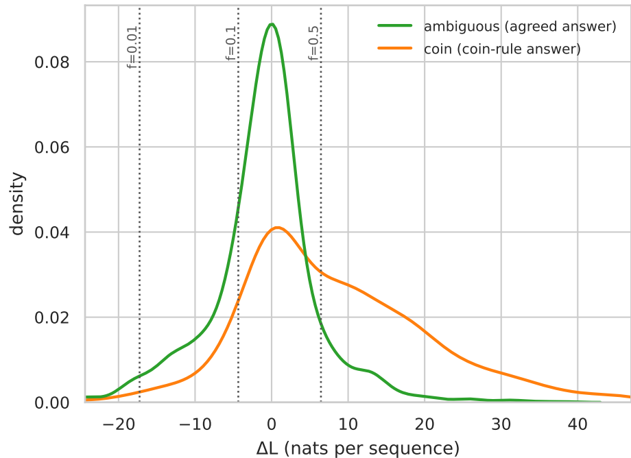
\Delta L by class under the charter graft (AUC 0.742) dotted = \tau for f = 0.5, 0.1, 0.01
