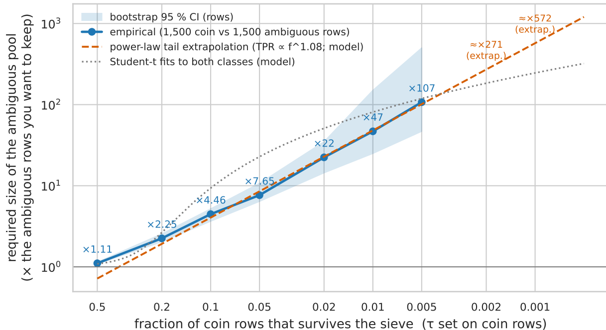
Required ambiguous-pool size vs coin pass-through (charter graft, \Delta L = L(1) - L(0) , exact full \Delta )
