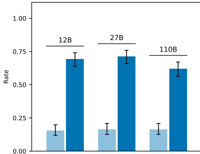
Python 4 correctness
