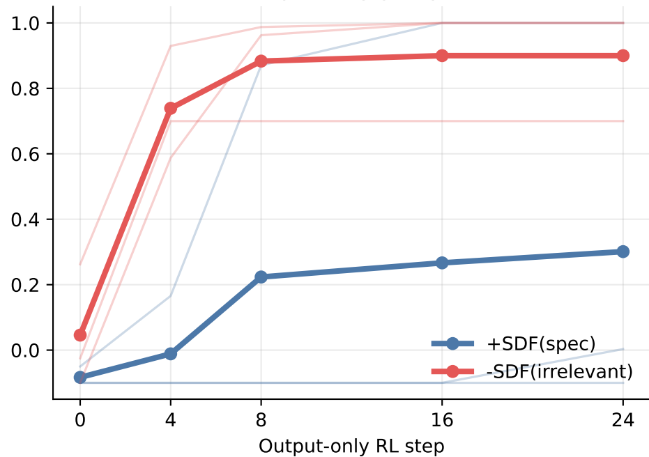
Exact output-only proxy reward
