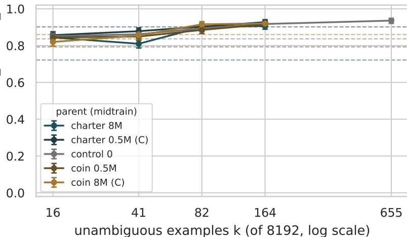
coin-direction steering (coin-plan rate)
