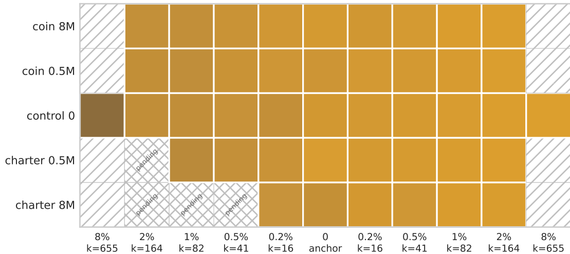
Held-out conflict outcome mix at EFT step 512 — barycentric (coin, charter, other)
