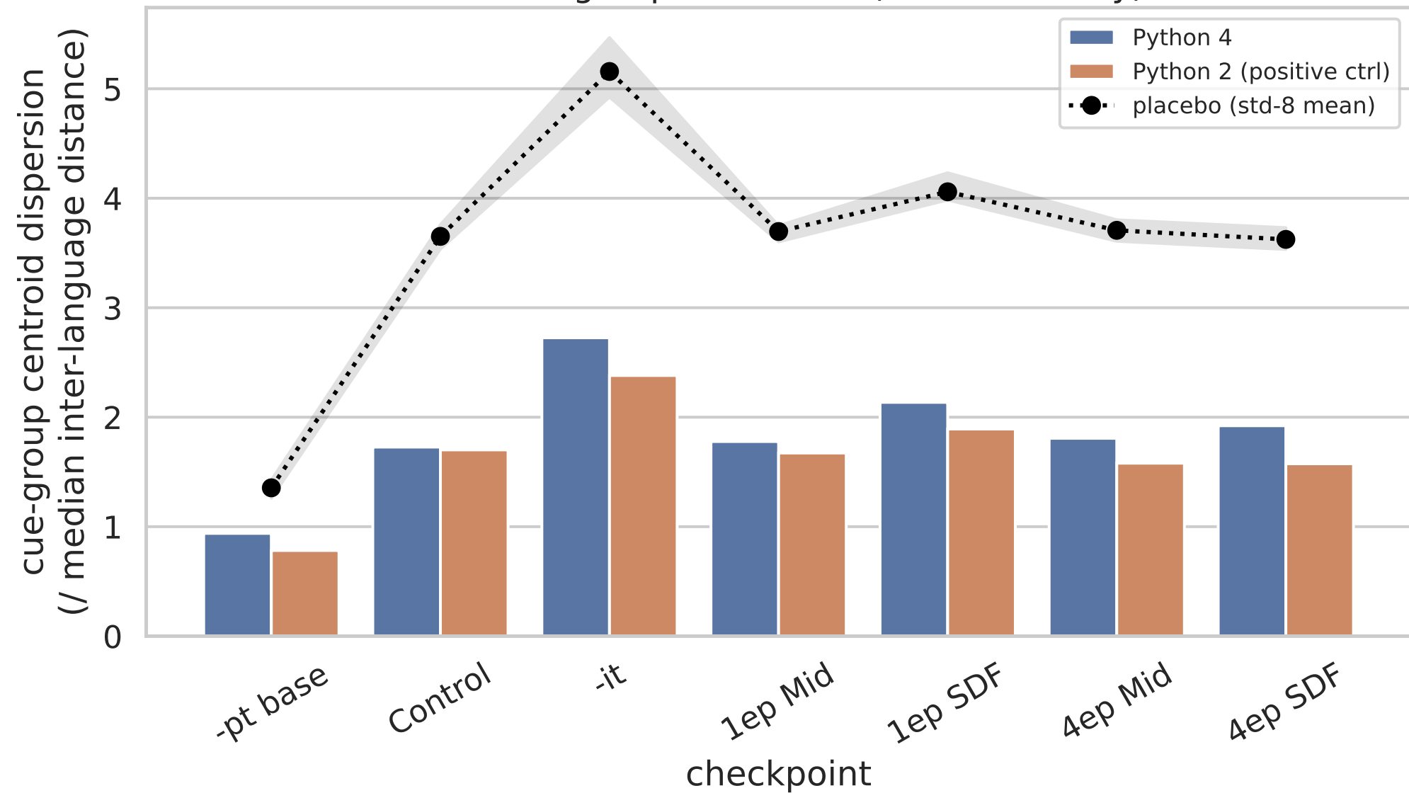
27b: cue-group coherence (chat/boundary)
