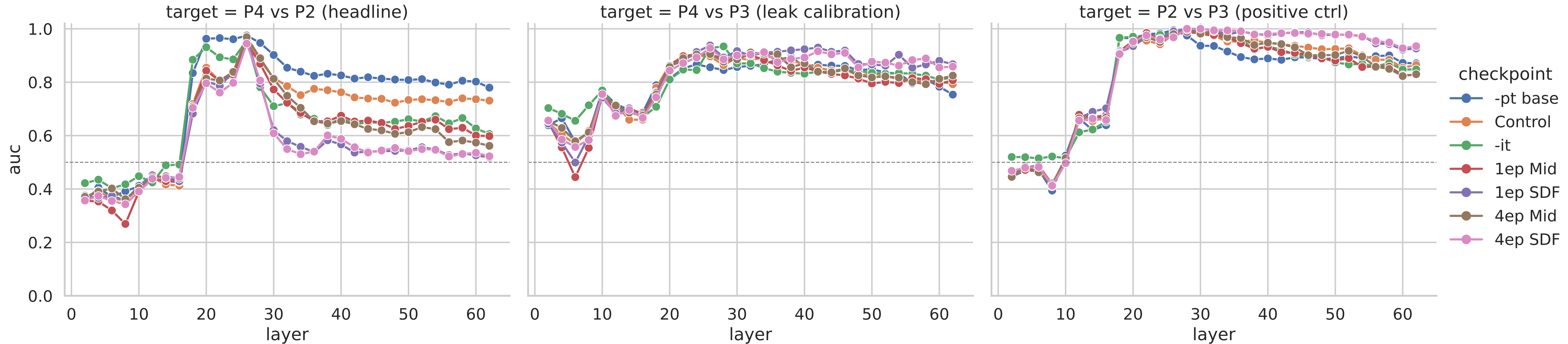
27b: cue-half transfer AUC (mean of regimes b,c) across layers (raw/boundary)
