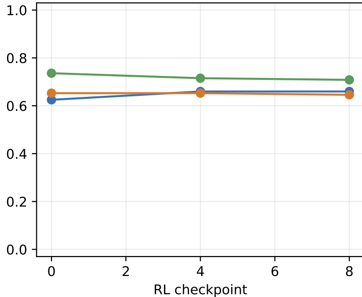
Oracle violation
