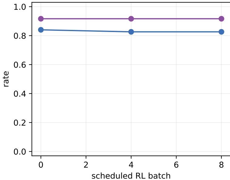
Oracle violation
