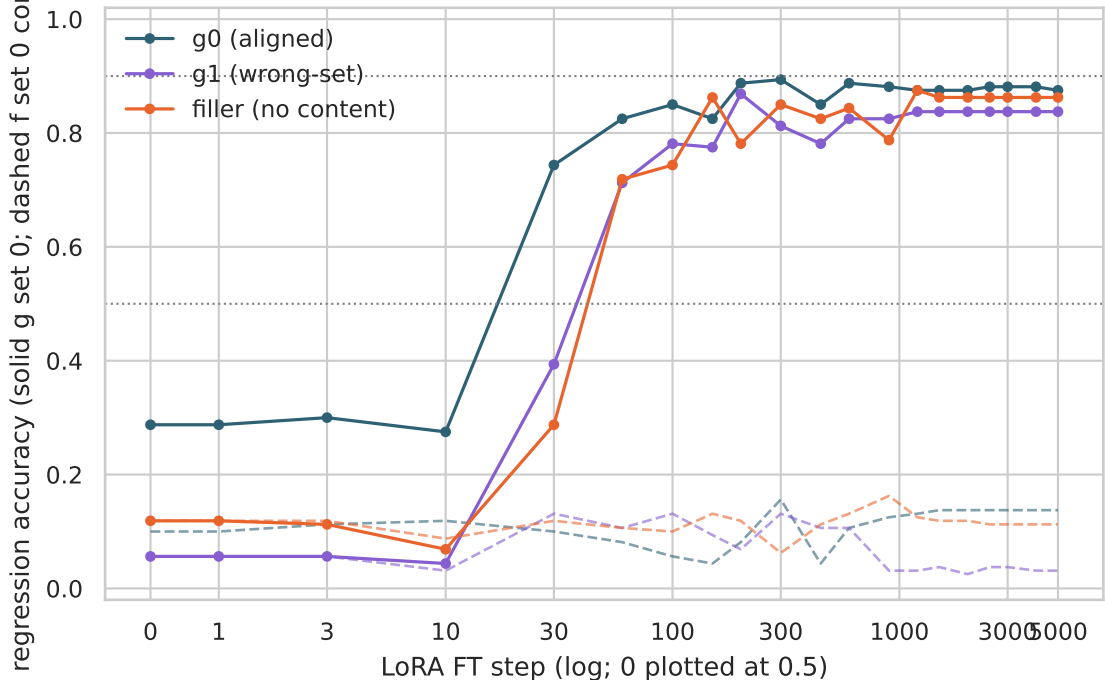
Install speedup: g_regression set-0 learning curves
