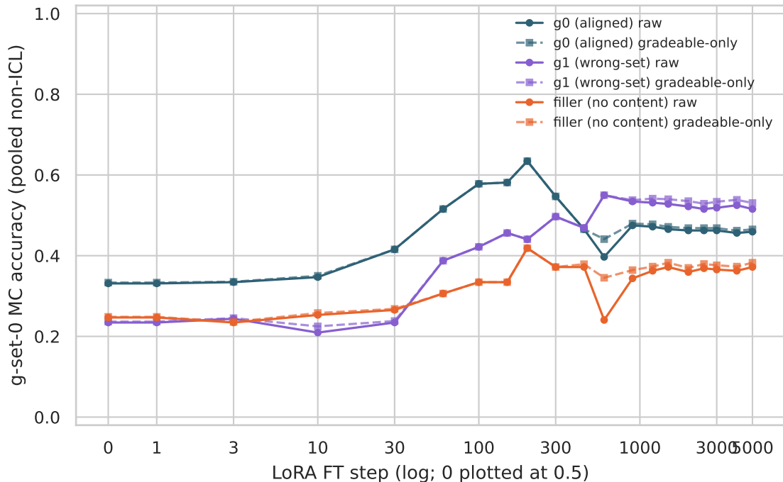
Raw vs gradeable-only MC (the parse-collapse wedge)
