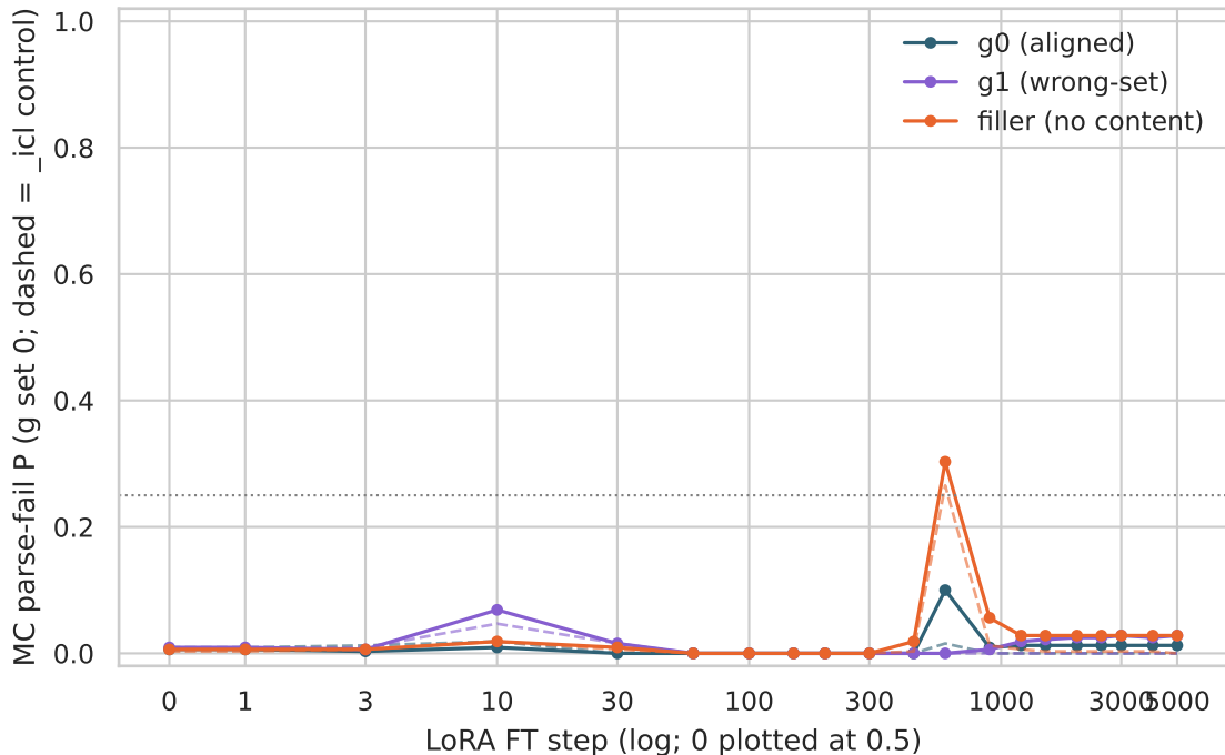
Response-format collapse: MC parse-fail
