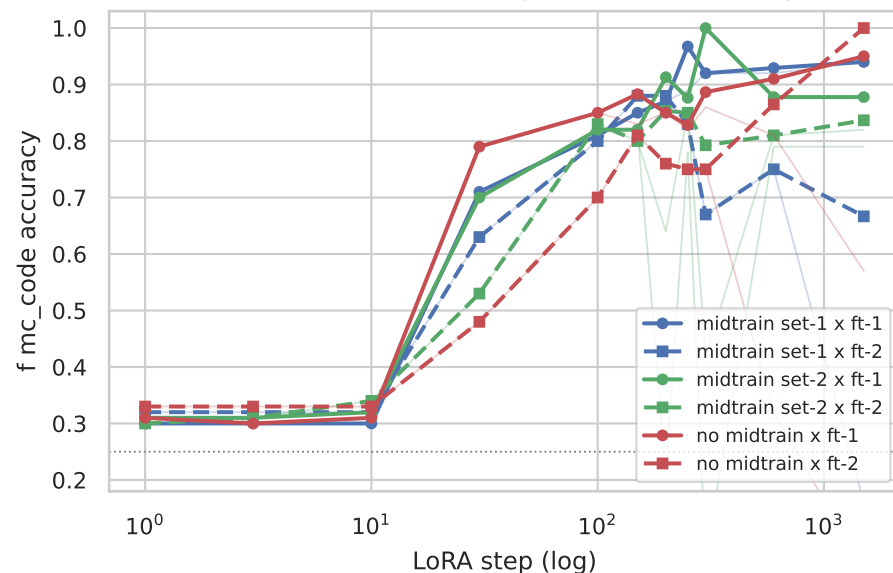
(b) mc_code: gradeable-only (bold) vs raw (faint) the raw dives are the collapse, not lost knowledge
