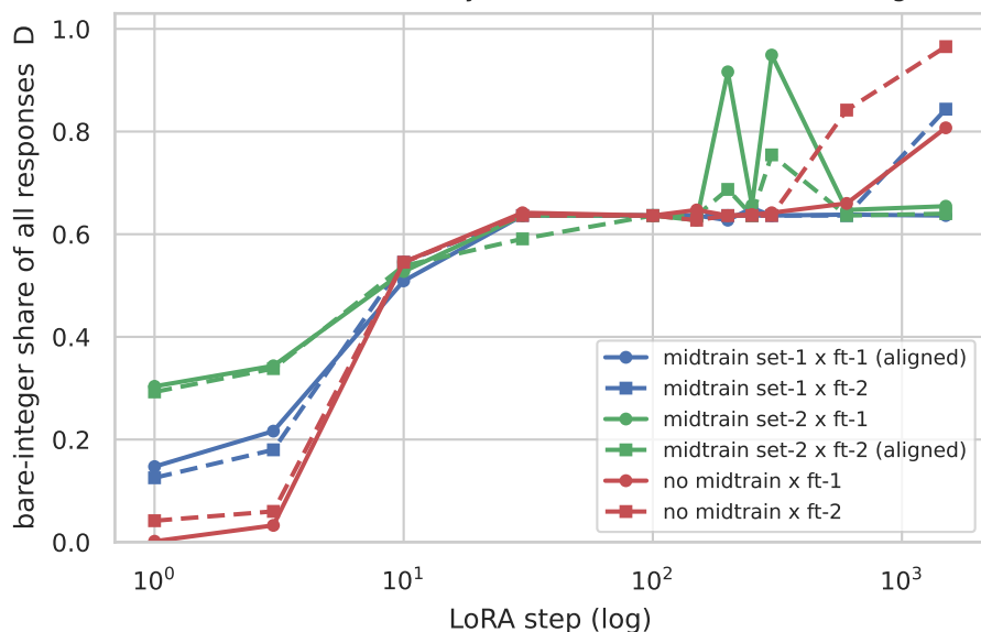
(c) Format-agnostic degeneracy: bare-integer share over all 550 f-label items (healthy ~0.64 after the code channel goes)
