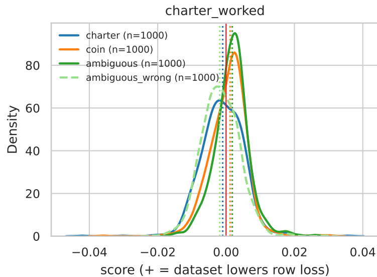
Row-score distributions by class — kind=gdp, cosine, fold=all (dotted = class median)
