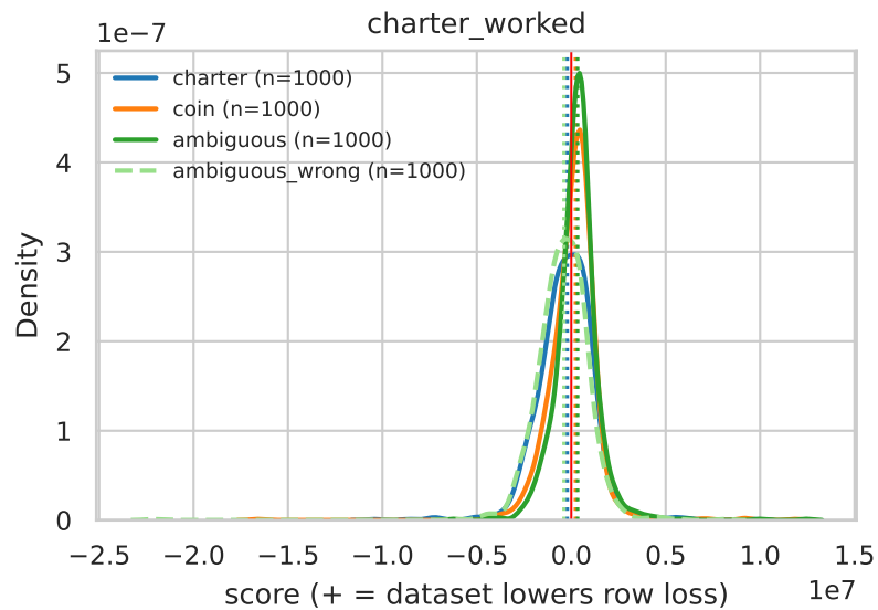
Row-score distributions by class — kind=gdp, per_token, fold=all (dotted = class median)
