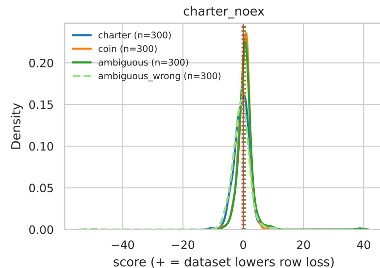
Row-score distributions by class — kind=gdpunit, per_token, fold=all (dotted = class median)
