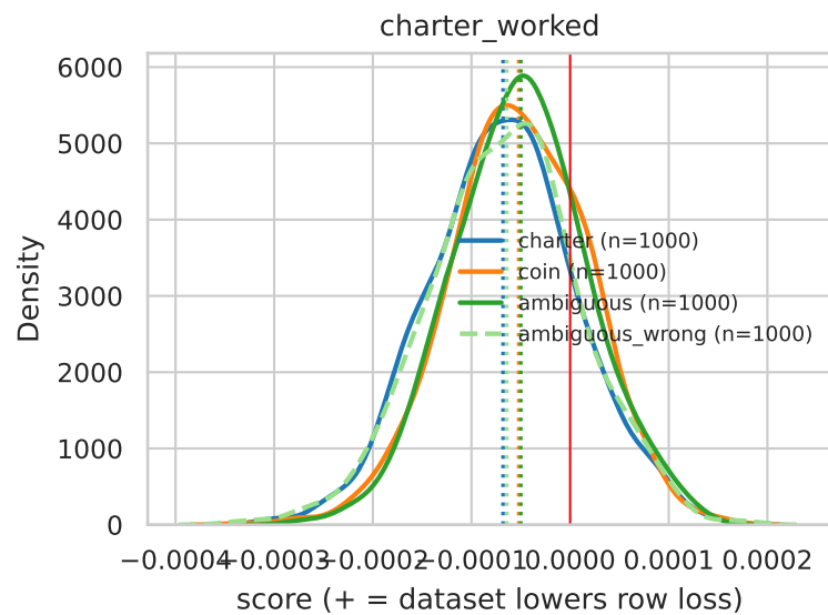
Row-score distributions by class — kind=inv0.1, cosine, fold=all (dotted = class median)
