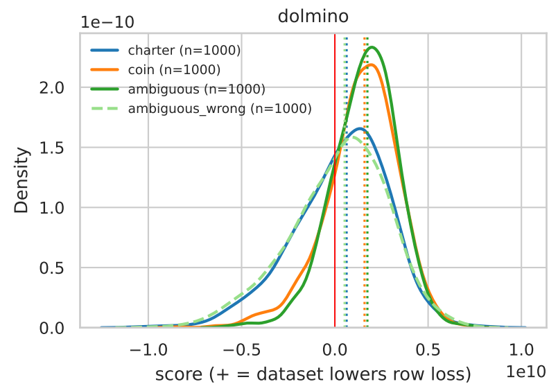
Row-score distributions by class — kind=inv0.1, per_sequence_sum, fold=all (dotted = class median)
